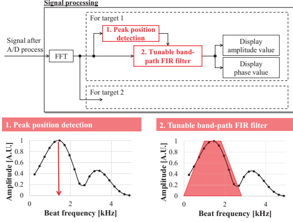
Figure 14: Block diagram of proposed multiple target detection in signal processing
