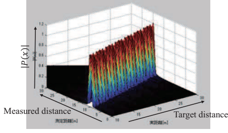
(a) 3D view.
