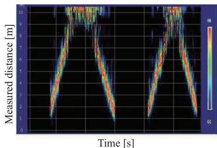
(b) With differential detection (Proposed)
