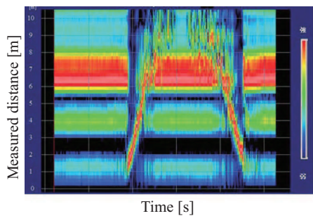
(a) Without differential detection
